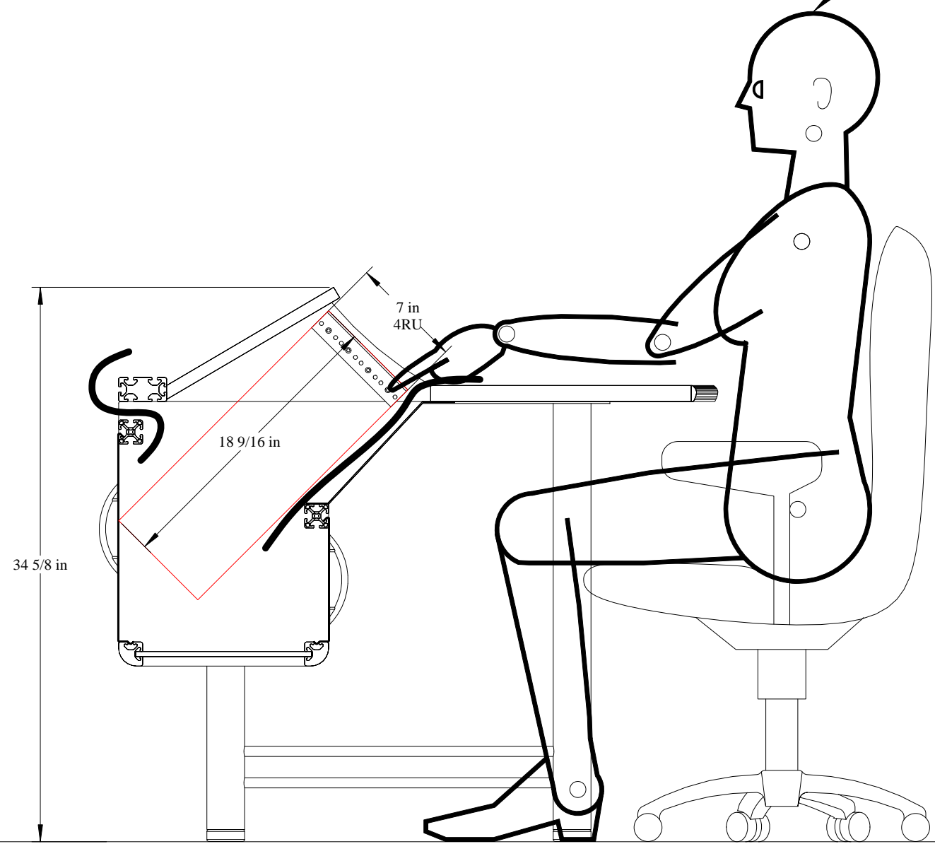
Section at 4RU equipment bay
